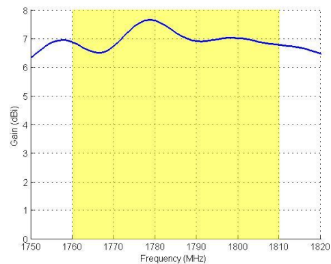
Gain
